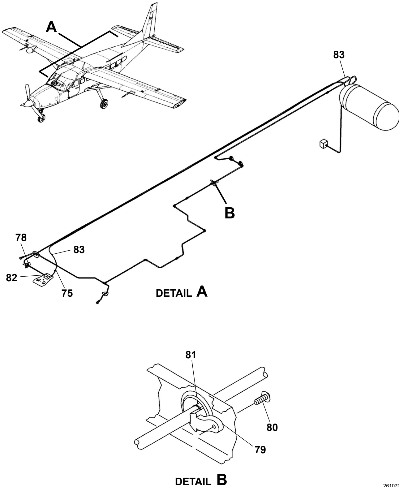
OXYGEN SYSTEM - 2 PORT PASSENGER VERSION Figure 04. (Sheet 2)
