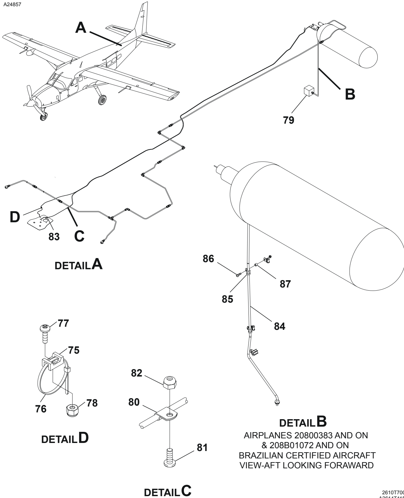
OXYGEN SYSTEM - 2 PORT Figure 02. (Sheet 2)
