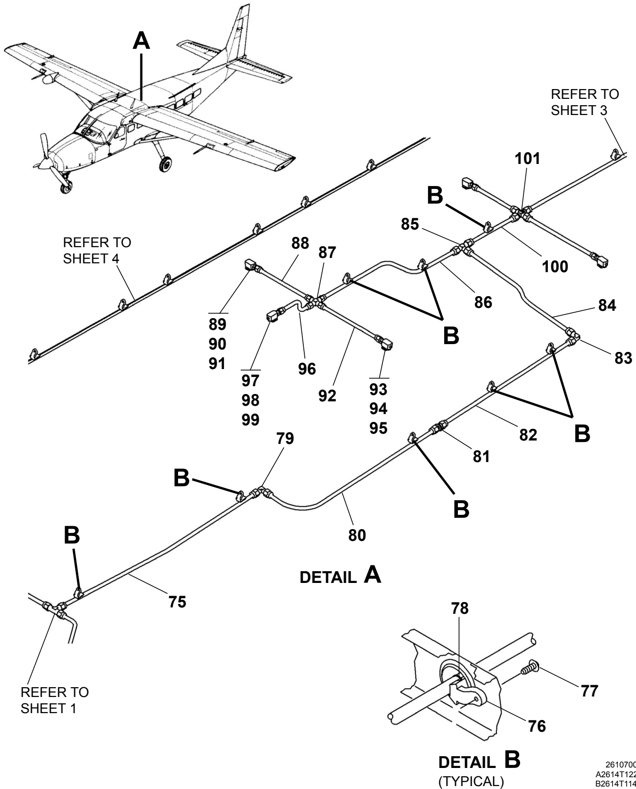
OXYGEN SYSTEM - 14 PORT PASSENGER VERSION Figure 04. (Sheet 2)
