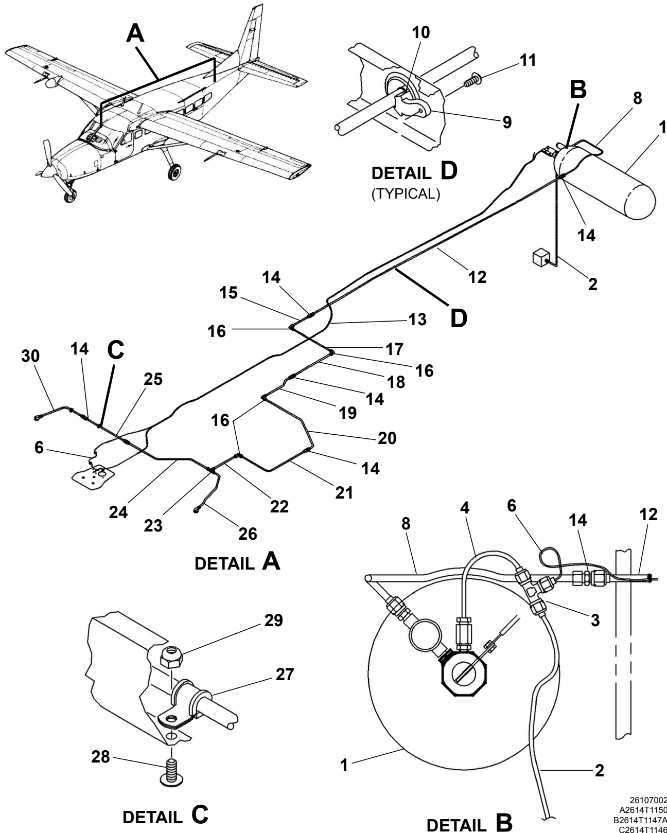
OXYGEN SYSTEM - 2 PORT Figure 02. (Sheet 1)
