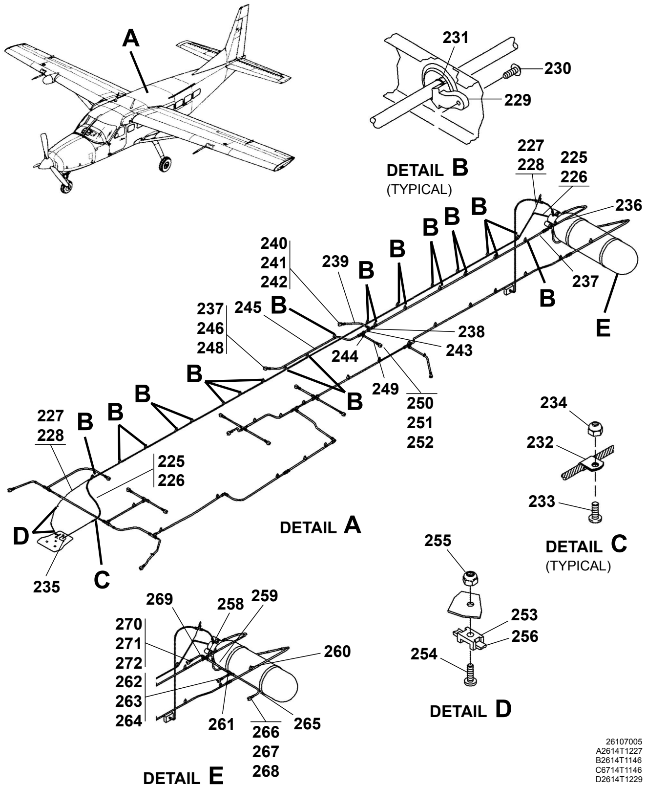
OXYGEN SYSTEM - 14 PORT PASSENGER VERSION Figure 04. (Sheet 4)
