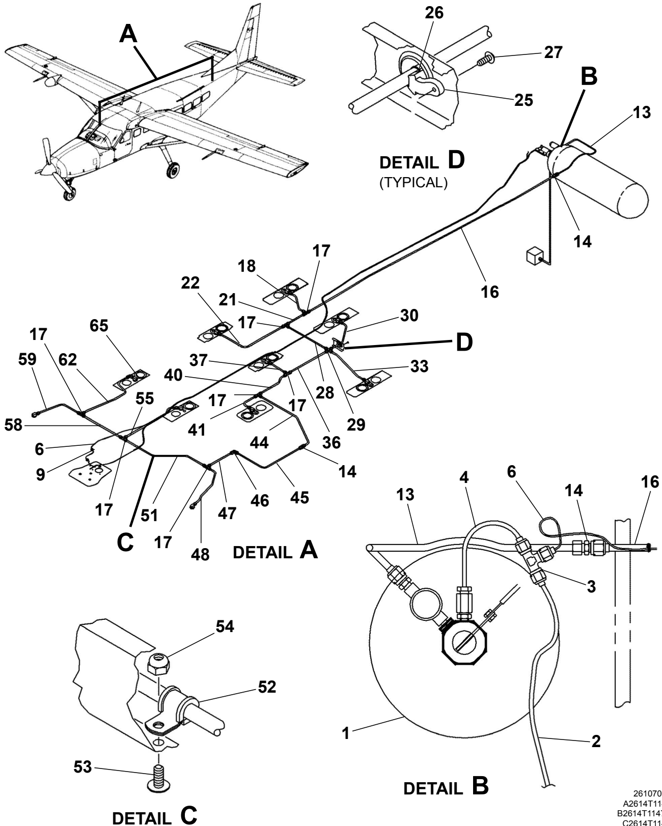
OXYGEN SYSTEM - 10 PORT Figure 02. (Sheet 1)
