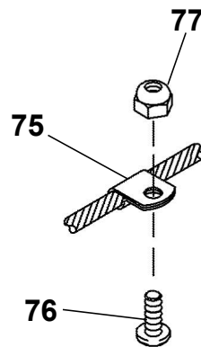
OXYGEN SYSTEM - 10 PORT Figure 02. (Sheet 2)
