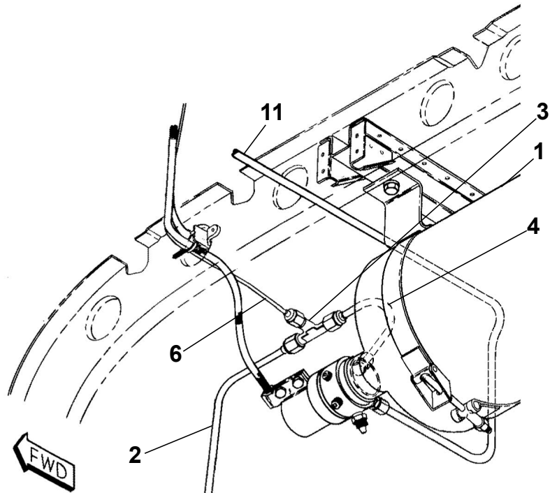
OXYGEN SYSTEM - 2 PORT Figure 01. (Sheet 1)
