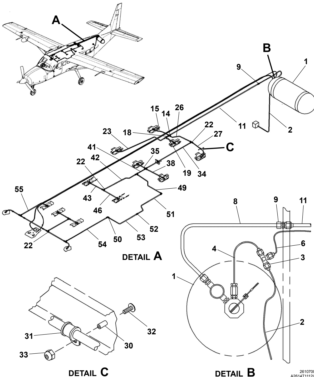
OXYGEN SYSTEM - 13 PORT PASSENGER VERSION Figure 03. (Sheet 1)
