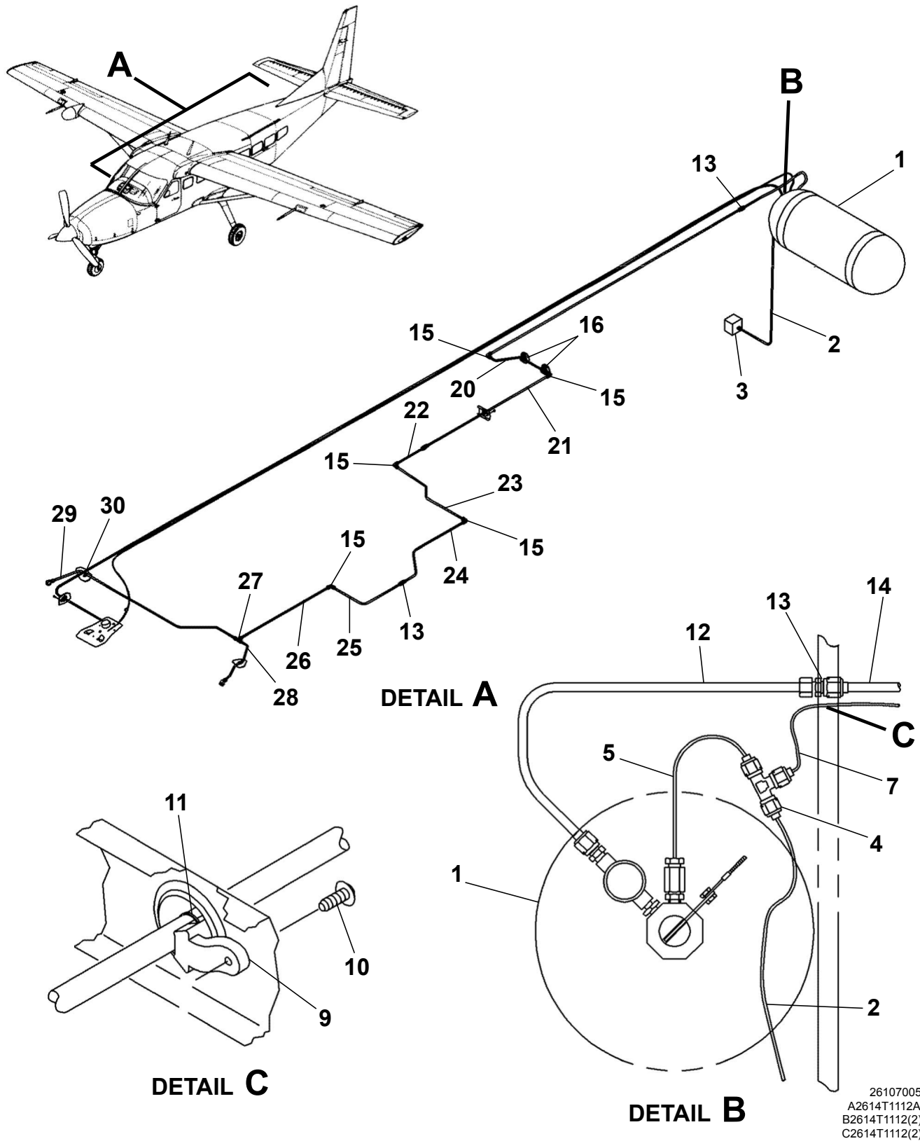
OXYGEN SYSTEM - 2 PORT PASSENGER VERSION Figure 04. (Sheet 1)
