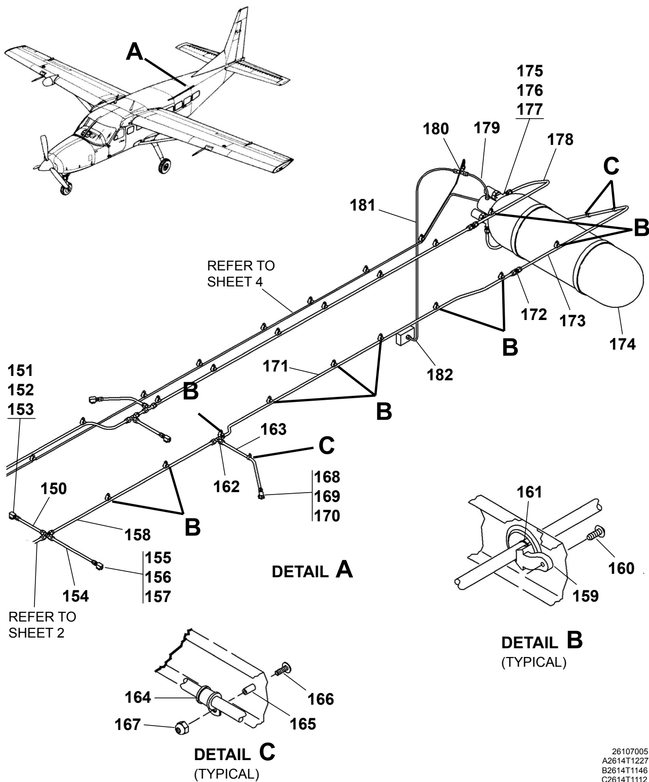
OXYGEN SYSTEM - 14 PORT PASSENGER VERSION Figure 04. (Sheet 3)
