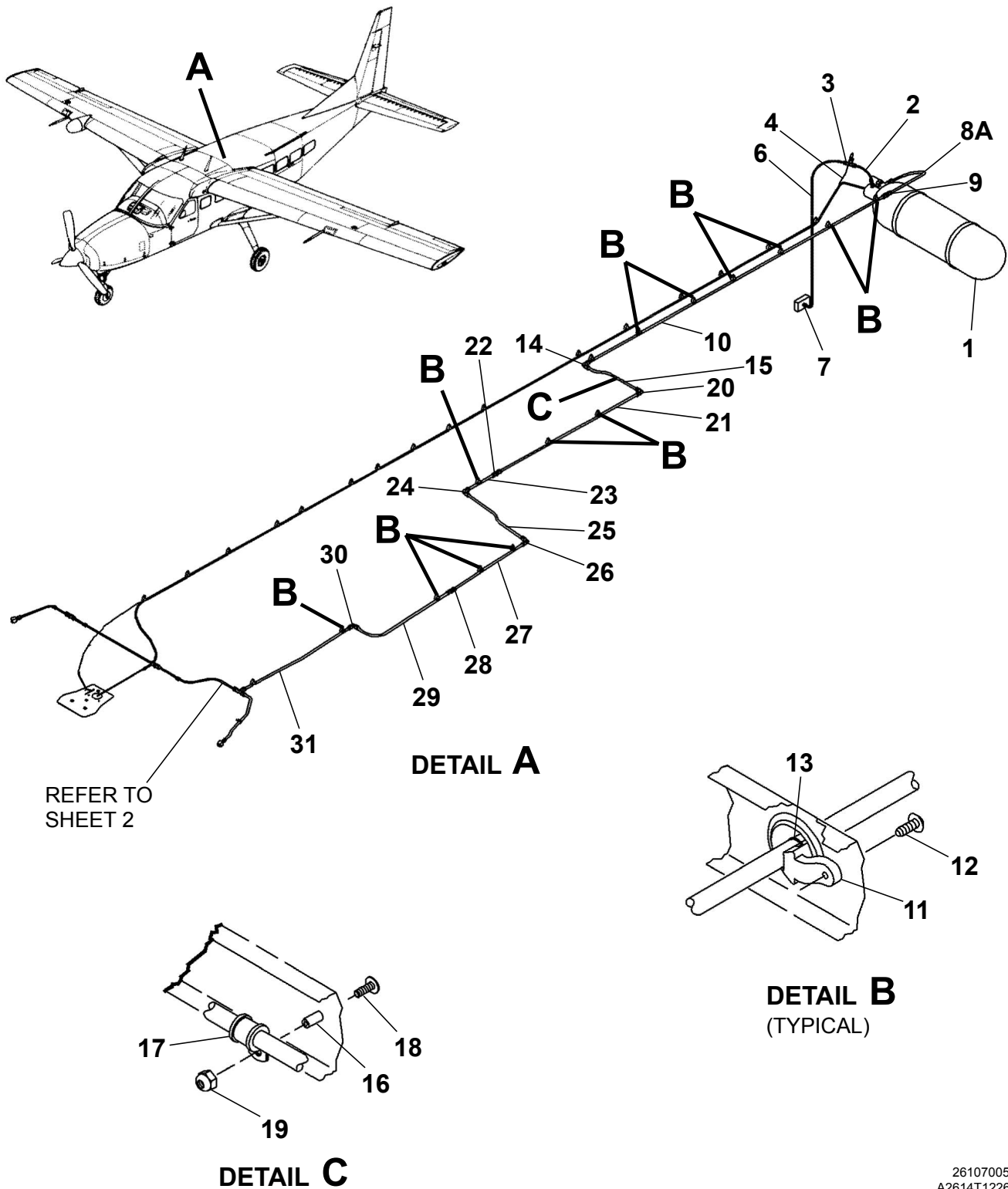
OXYGEN SYSTEM - 2 PORT PASSENGER VERSION Figure 05. (Sheet 1)
