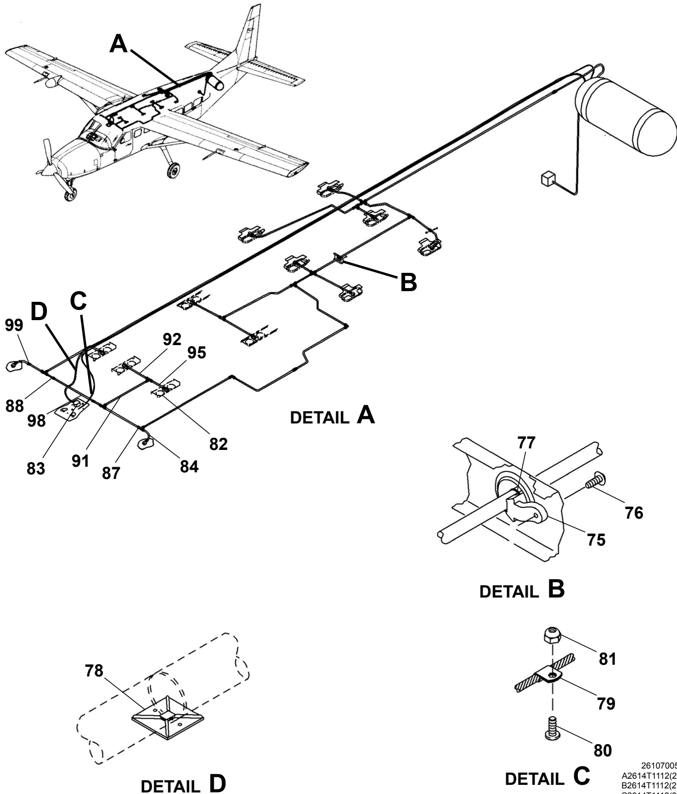
OXYGEN SYSTEM - 13 PORT PASSENGER VERSION Figure 03. (Sheet 2)
