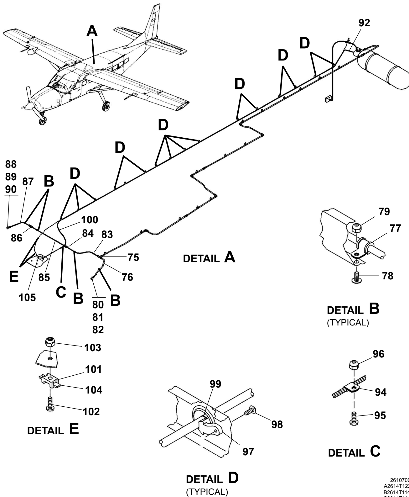
OXYGEN SYSTEM - 2 PORT PASSENGER VERSION Figure 05. (Sheet 2)
